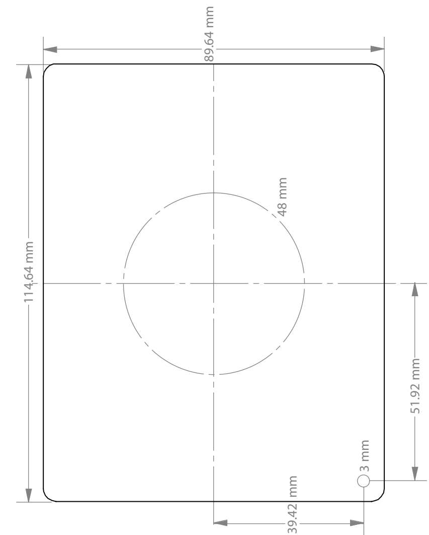
Figure 2 Truecharge2 Remote Panel Mounting Template (1:1)
