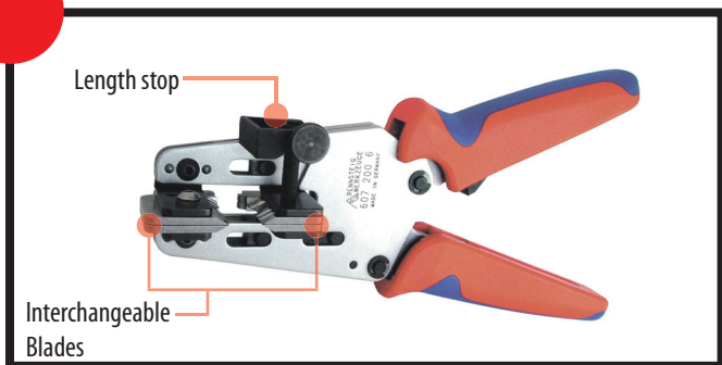
Insulation Stripper
