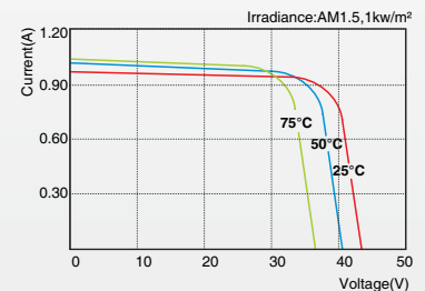
SLP030-24U I-V Curves
