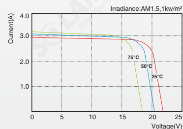
SLP045-12U I-V Curves
