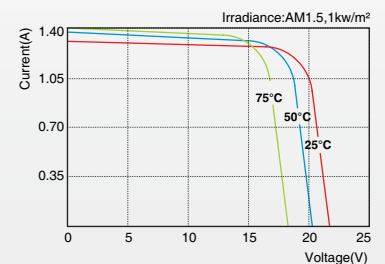
SLP020-12U I-V Curves
